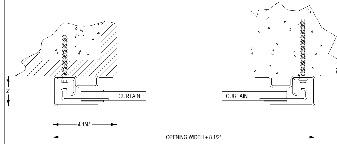
FIGURE 12: CONCRETE / MASONRY JAMBS
