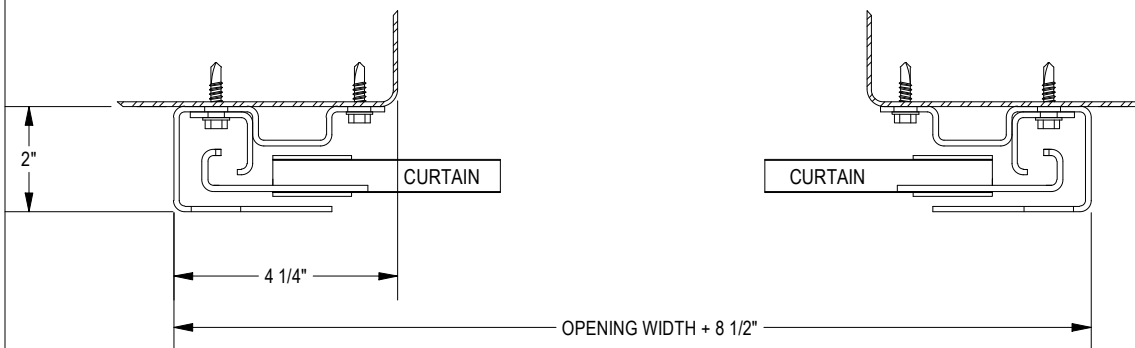
FIGURE 14: STEEL JAMBS
