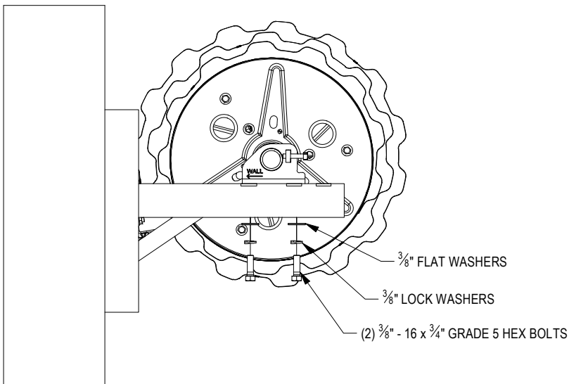
FIGURE 16: SECURING STAMPED AXLE SUPPORT TO BRACKETS
