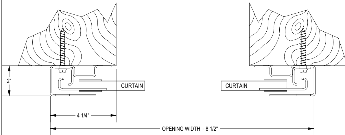
FIGURE 13: WOOD JAMBS
