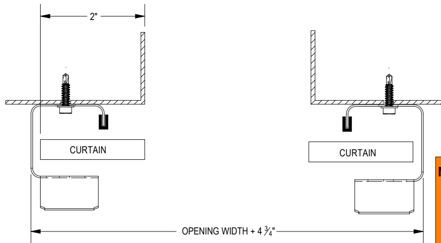
FIGURE 17: STEEL JAMBS
