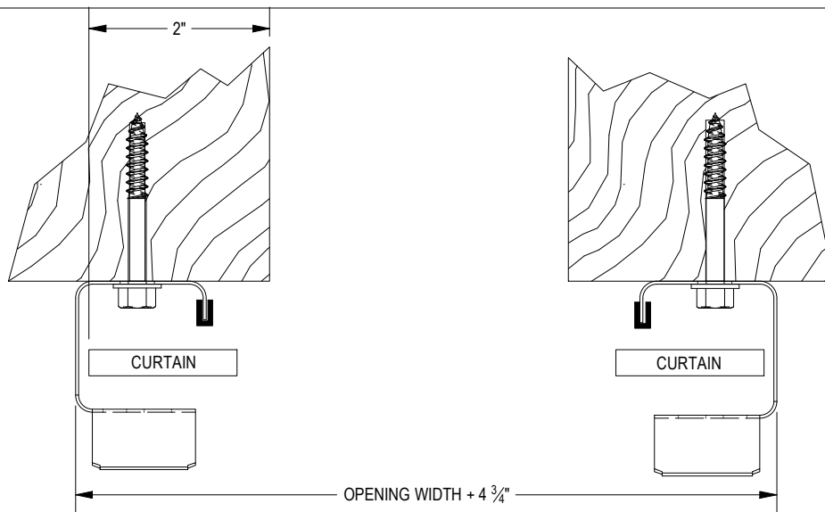
FIGURE 19: WOOD JAMBS
