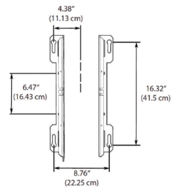
Bracket mounting
