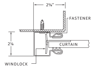
Model 283 - Windlock (for opening widths over 6'0" through 10'0")
