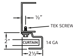
201HD Standard Guide Mount to Steel
