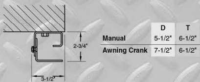
Face of Wall Mount
