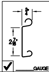
GAUGE
