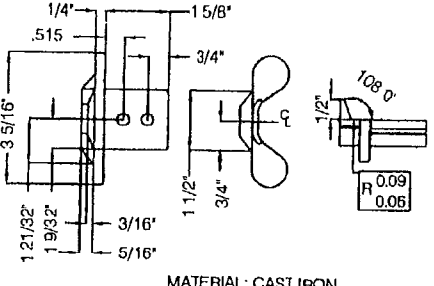
MATERIAL: CAST IRON WINDLOCK
