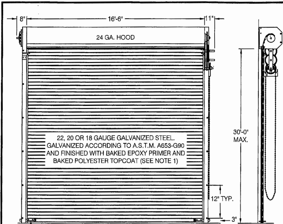
INTERIOR ELEVATION SIDE ELEVATION
