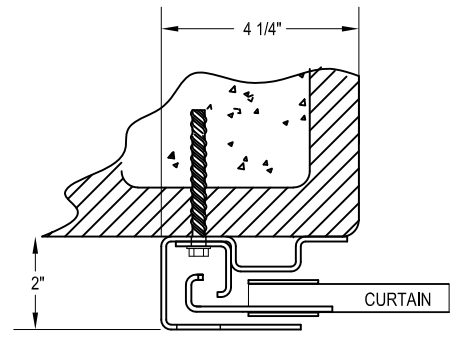
CONCRETE FILLED JAMB: (OPTION 2) 3/8" x 4" DEWALT WEDGE BOLT + SCREW ANCHORS
