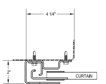
STEEL JAMB (OPTION 3) STEEL JAMBS USING 1/4" - 14 X 1" SELF DRILLING SCREW
