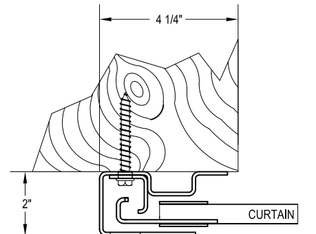
WOOD JAMB: (OPTION 2) 3/8" X 3" LAG BOLTS
