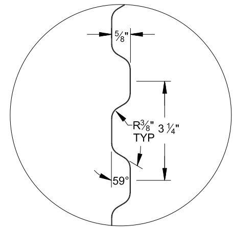
STEEL JAMB (OPTION 3) STEEL JAMBS USING 1/4" - 14 X 1" SELF DRILLING SCREW
